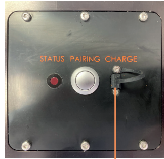
USB Charging Port
